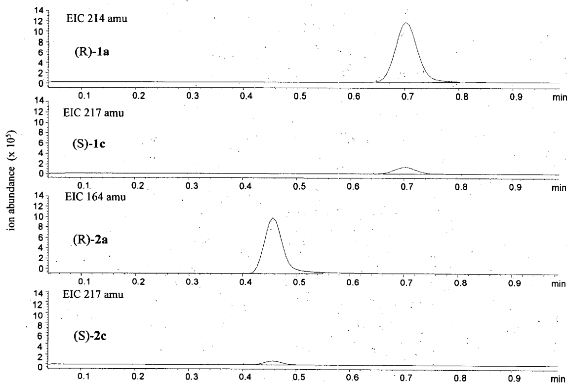
Figure Simultaneous determination of enantioenrichment of two different isotopically differentiated pseudoenantiomers. Conditions as in Figure 1.
